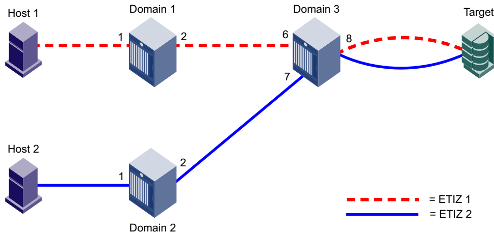
FIGURE 38 Enhanced TI zones
